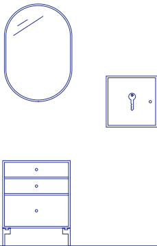
Mirror D 1.6 cm W 46.8 cm H 69.6 cm Shelving D 30 W 46.8 cm H 46.8 cm Legs H 12.6 cm Shelving D 20 cm W 35.4 cm H 35.4 cm
