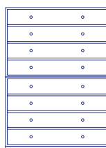
Dresser on plinth D 38 cm W 69.6 cm H 93.6 cm Plinth H 3 cm
