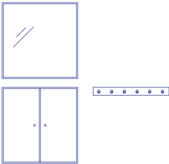
Mirror D 1.6 cm W 69.6 cm H 69.6 cm Shelving D 30 cm W 69.6 cm H 69.6 cm Rack D 5.4 cm W 69.6 cm H 10 cm
